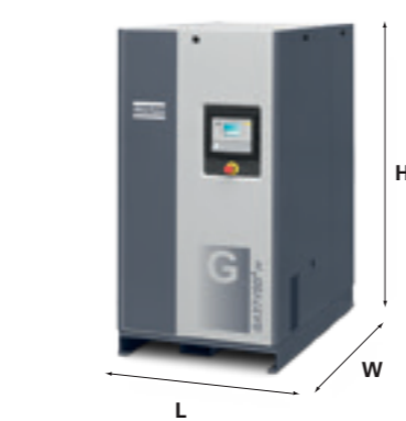
GA 15 VSD+ (STANDARD/FULL FEATURE) H: 1420 mm, 56" L: 630 mm, 25" W: 610/985 mm, 24/39" GA 18-37 VSD+ (STANDARD/FULL FEATURE) H: 1590 mm, 63" L: 780 mm, 31" W: 811/1273 mm, 32/50"
